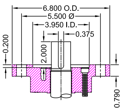
TOP MOUNTING FLANGE DIMENSIONS
